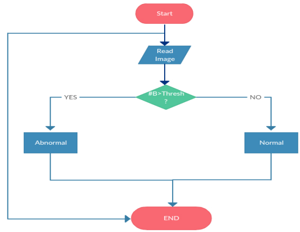
Fig.8 Binarization check method flowchart
